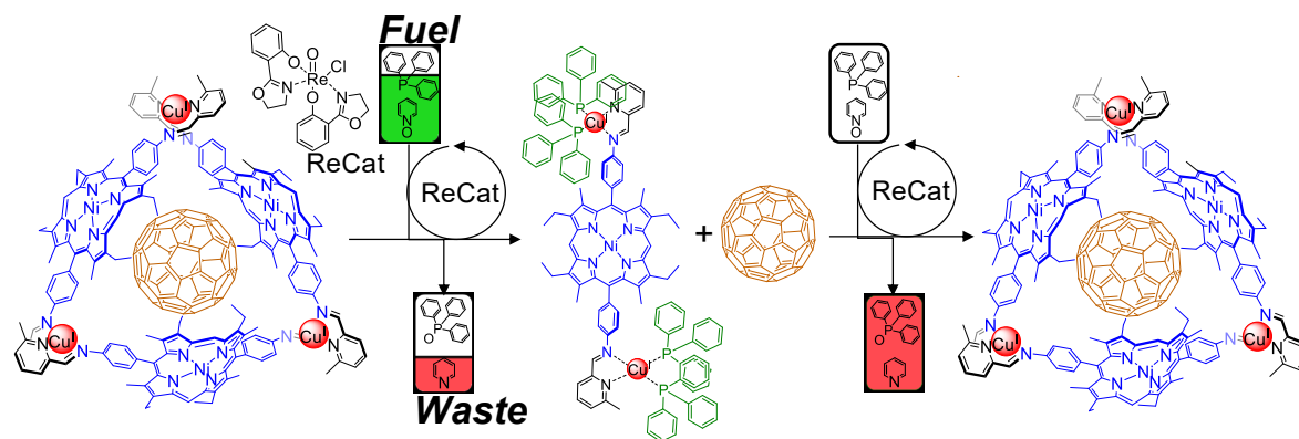
Figure 2. A system wherein the duration of release of a guest ( \text{C}_{60} ) can be programmed by the amount of fuel ( \text{PPh}_3 ) present
