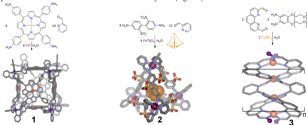
Figure 1. \text{Fe}^{\text{II}}_8 cubic cage 1 , 1 \text{Fe}^{\text{II}}_4 tetrahedral cage 2 , 2 and electroluminescent \text{Cu}^{\text{I}}_n double-helical polymer 3 3
